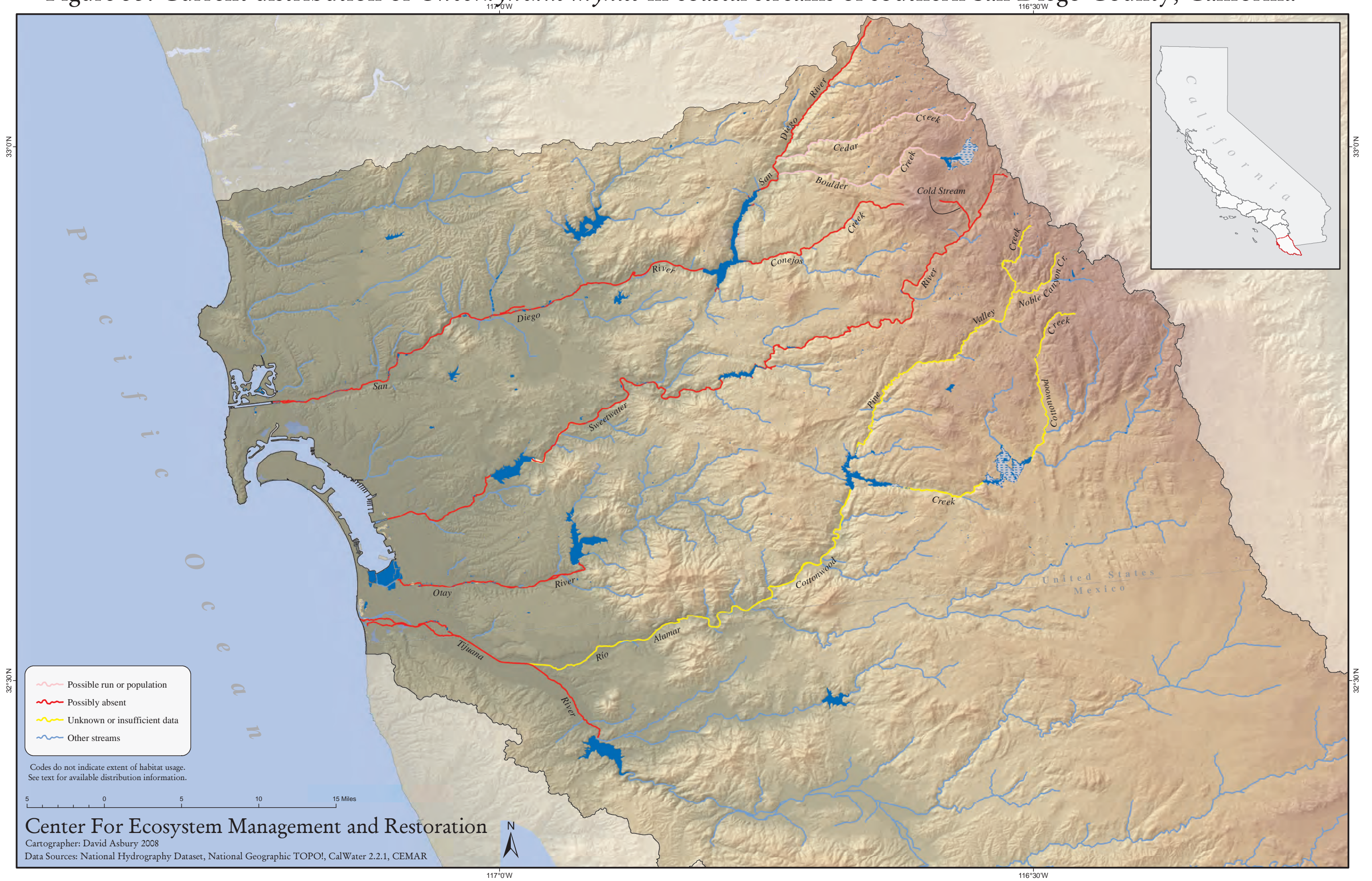
Figure 35. Current distribution of Oncorhynchus mykiss in coastal streams of southern San Diego County, California
