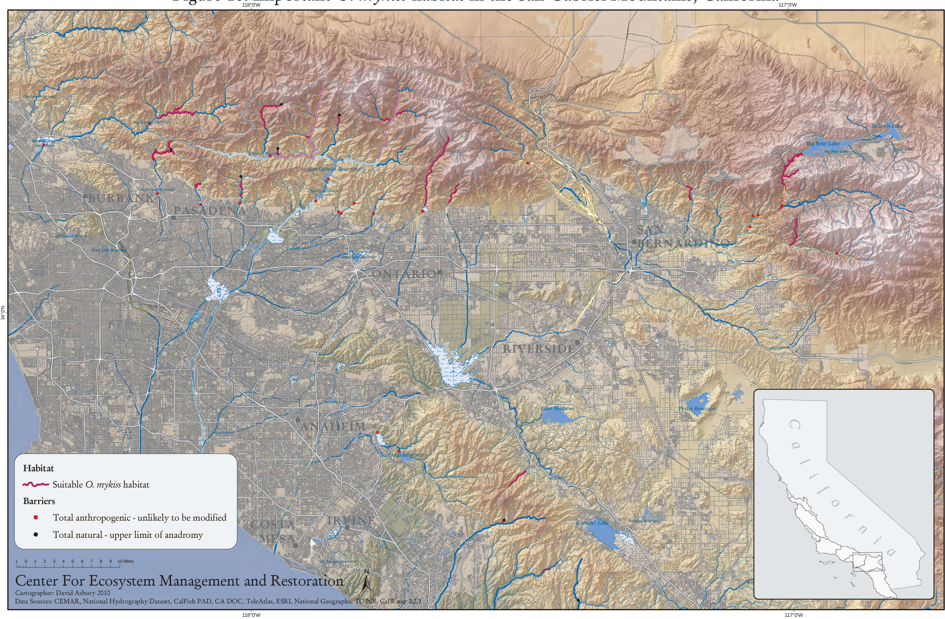
Figure 16. Important O. mykiss habitat in the San Gabriel Mountains, California
