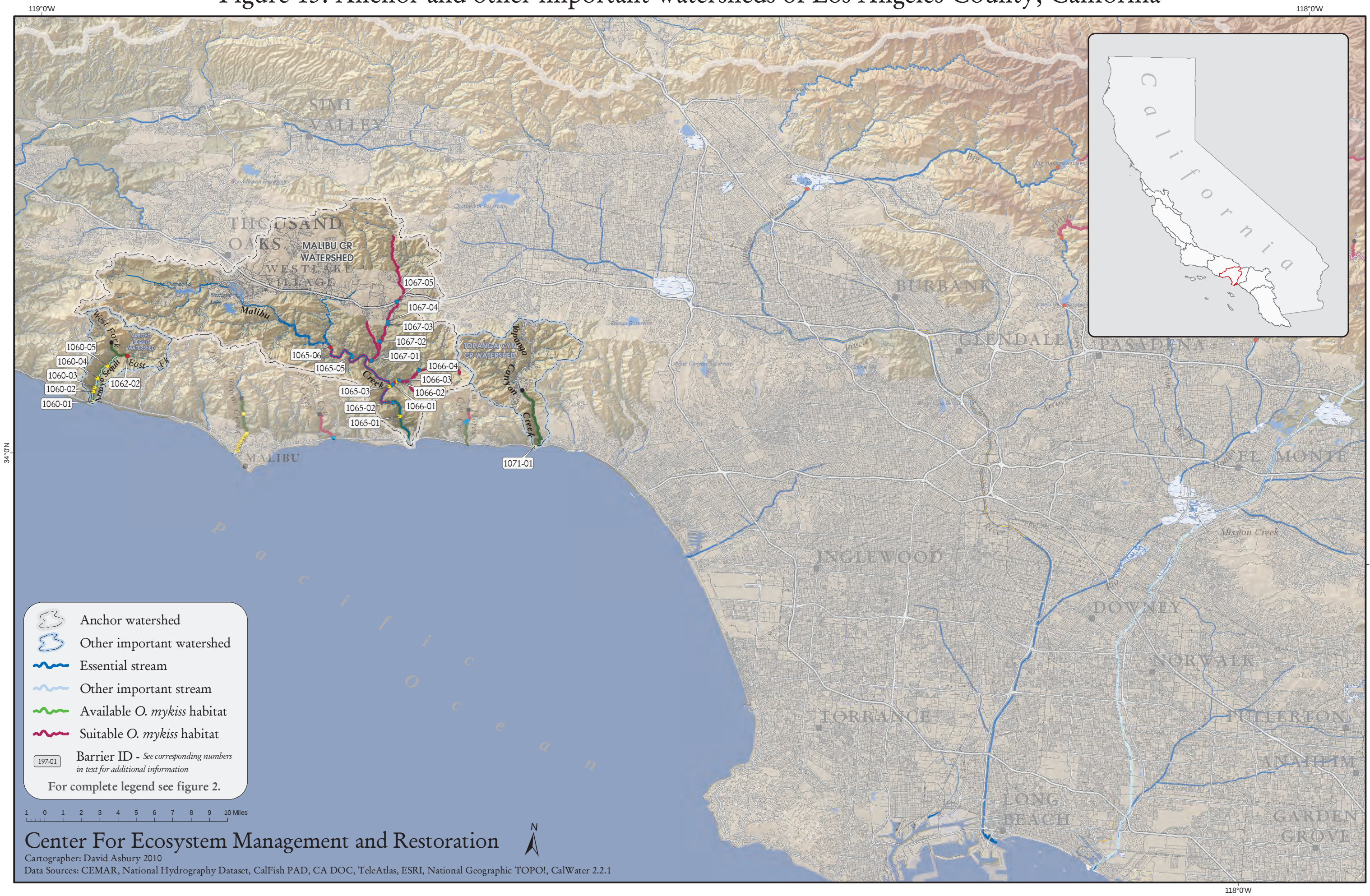
Figure 15. Anchor and other important watersheds of Los Angeles County, California
